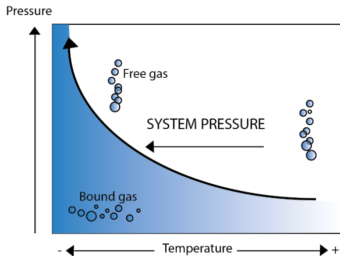
Figure 5. Solubility of air in fluids
